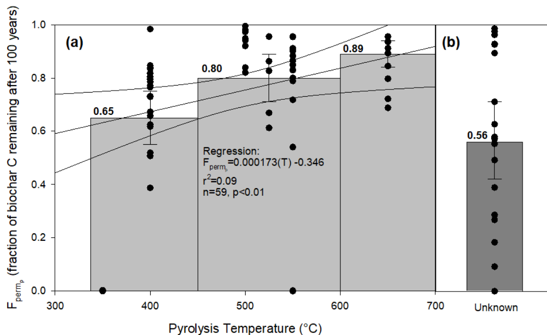
Figure 4A.1 F_{\text{perm}} calculated from field and laboratory studies for biochars that were made under different conversion conditions: (a) F_{\text{perm}} estimated for biochars with known production temperatures by fitting a two-pool double-exponential model to 59 datasets from eight mineralization experiments that exceeded one year and allowed a two-pool model to be fitted and adjusted to a decomposition temperature of 20°C recalculated as shown in Lehmann et al. (2015) (Sources of data include: Major et al. 2010; Zimmerman 2010; Singh et al. 2012; Zimmerman & Gao 2013; Fang et al. 2014; Herath et al. 2015; Kuzyakov et al. 2014; Dharmakeerthi et al. 2015; Wu et al. 2016); (b) F_{\text{perm}} estimated for naturally occurring chars and added biochars with unknown production temperatures using 20 observations from eight long-term field assessments (decadal to millennial time scales) where physical export is not determined (Cheng et al. , 2008; Hammes et al. , 2008; Lehmann et al. , 2008; Liang et al. , 2008; Nguyen et al. , 2008; Vasilyeva et al. , 2011; Lutfalla et al. , 2017; mean residence times taken directly from the sources without recalculation).
